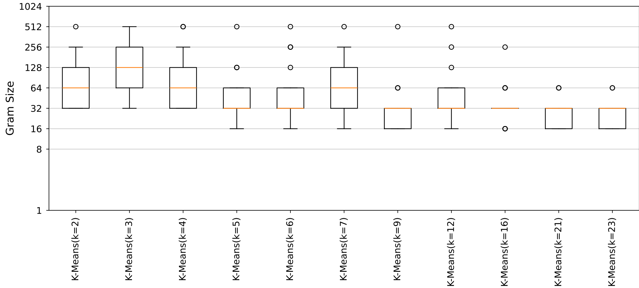
YARA Rules Gram Size Distribution (Cluster5_Size23 dataset)
